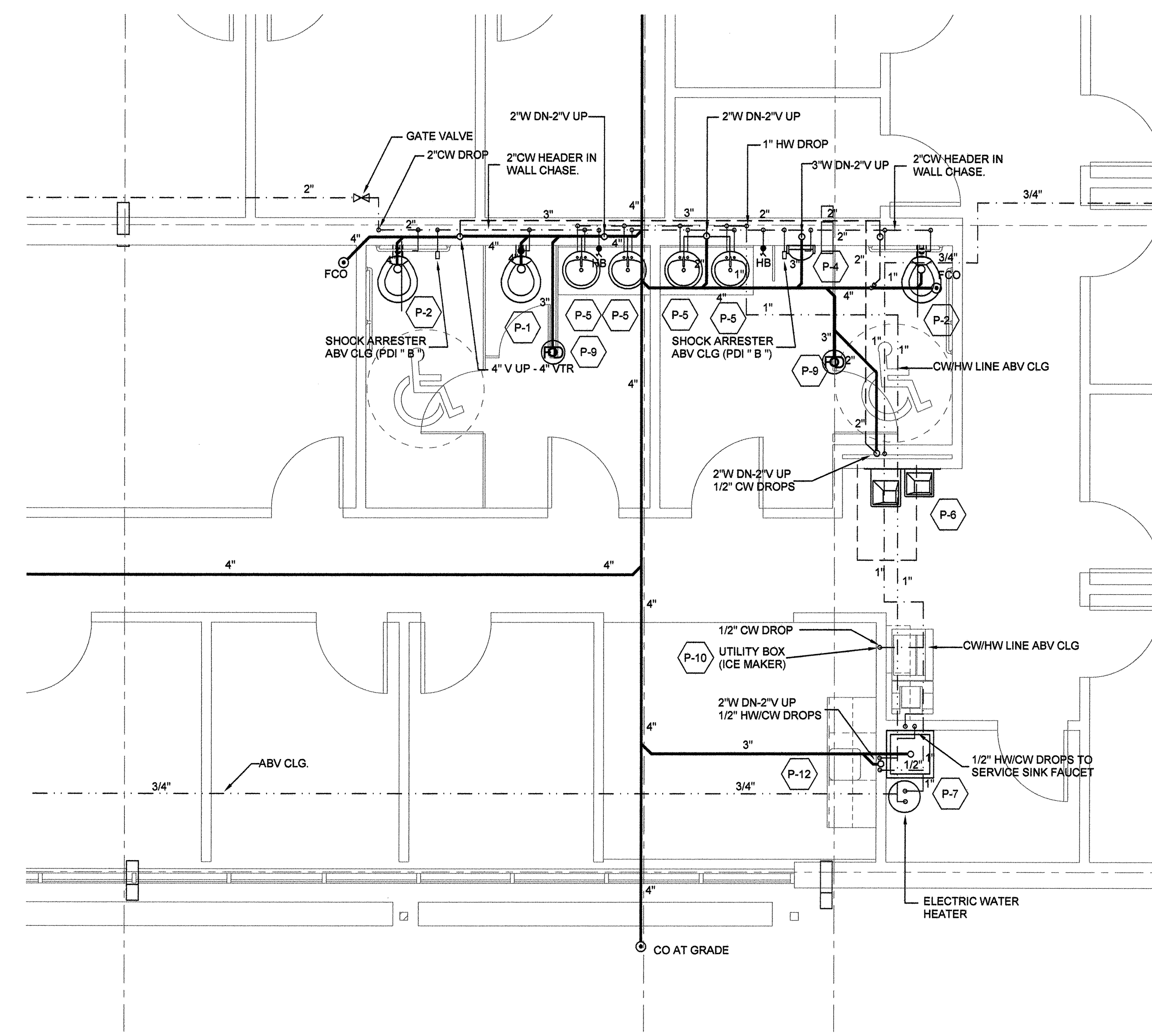
2 ENLARGED PLUMBING PLAN - TOILETS 118 & 119 P-2 SCALE: 1/4" = 1'-0"
